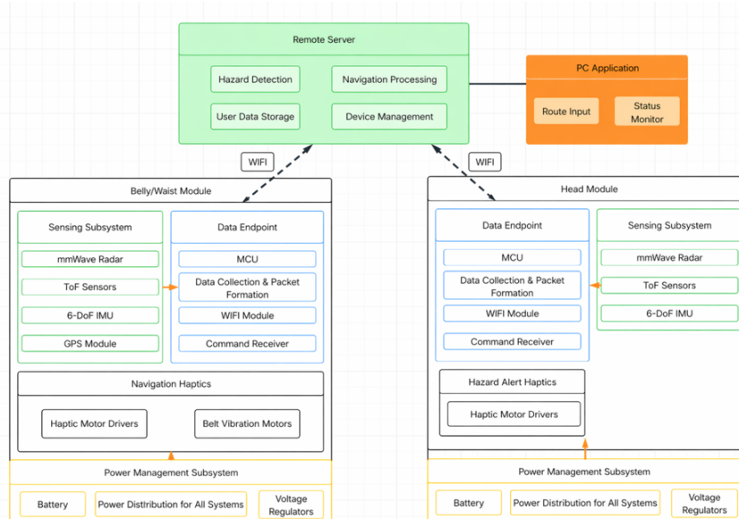
Figure 1: Top-level system block diagram. Each wearable module bundles a sensing block (ToF, mmWave, IMU, plus GPS on the waist module), an MCU-based control block, and a haptic output block; both modules share a host running the fusion algorithm and the Maps-based navigation frontend.
